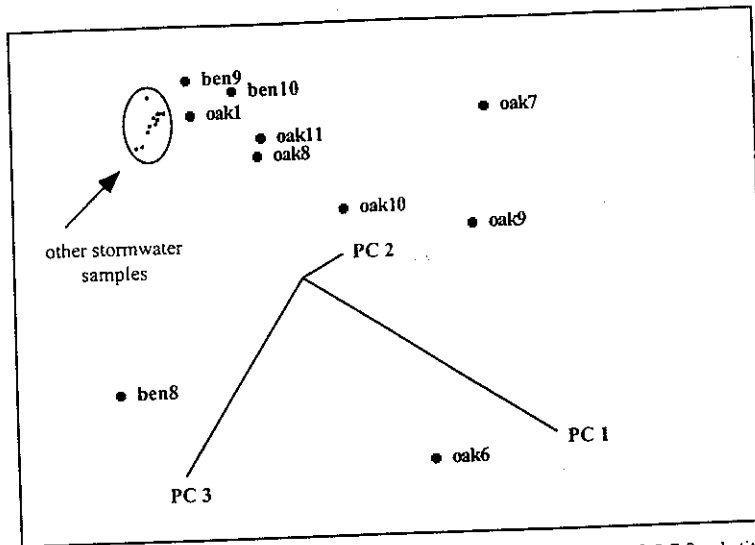
Fig. 1: Three dimensional principal components scores plot of normalized 2,3,7,8-substituted PCDD/Fs in urban stormwater samples collected hourly during the first major rainfall of the winter season from outfalls located in the cities of Oakland (oak) and Benicia (ben), California. Results indicate that the PCDD/F content in stormwater changed significantly 6 hrs (oak6 - oak11) and 8 hrs (ben8 - ben10) after collection of the first samples.
